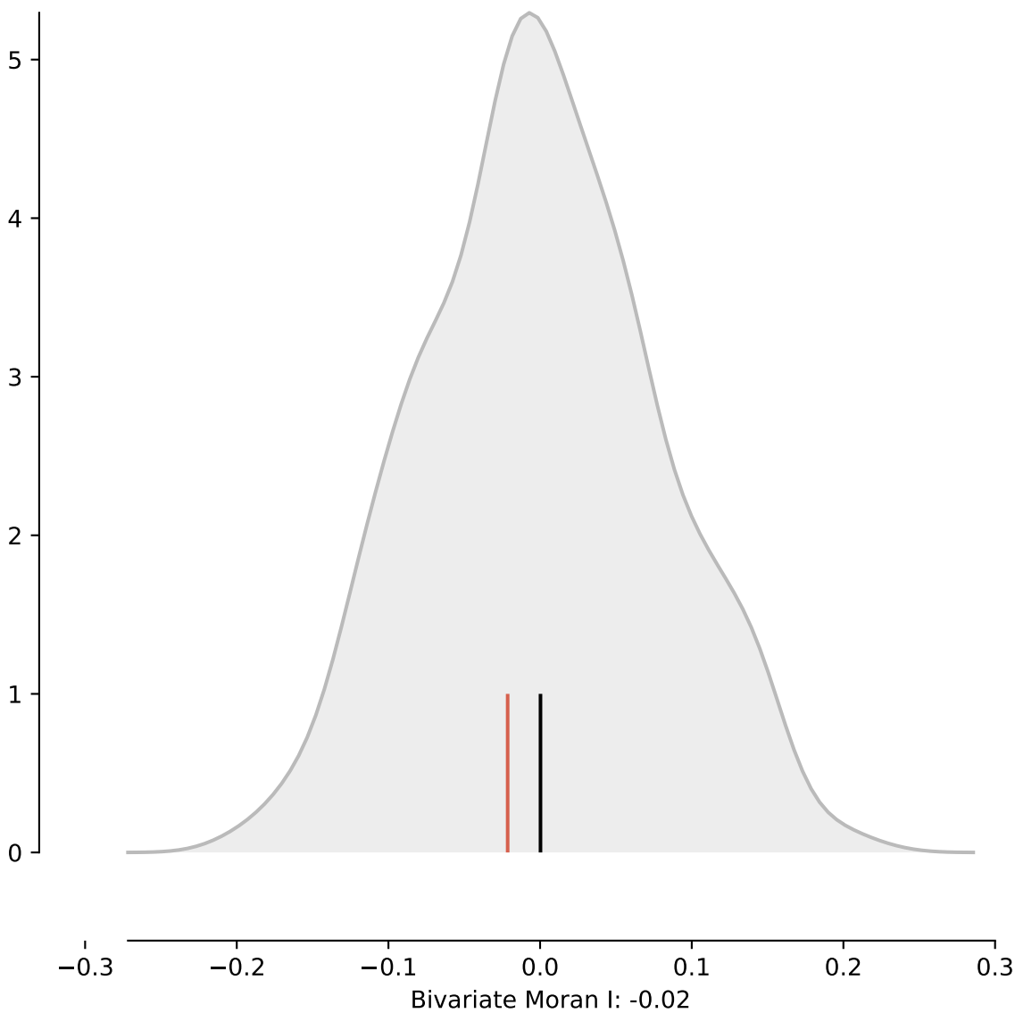
Reference Distribution
