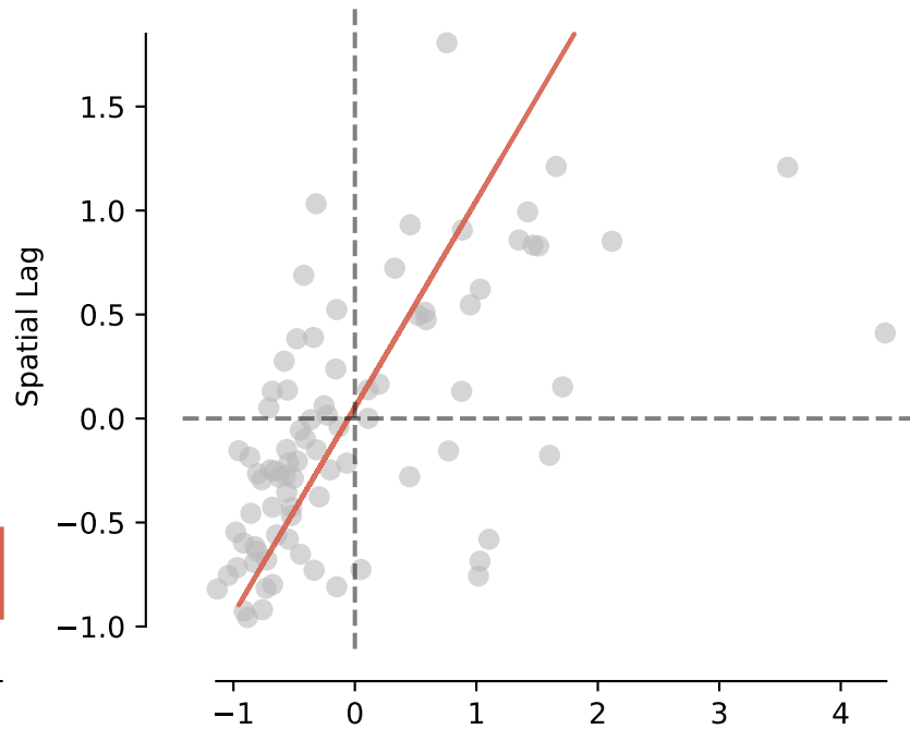
Moran Scatterplot (0.35)
