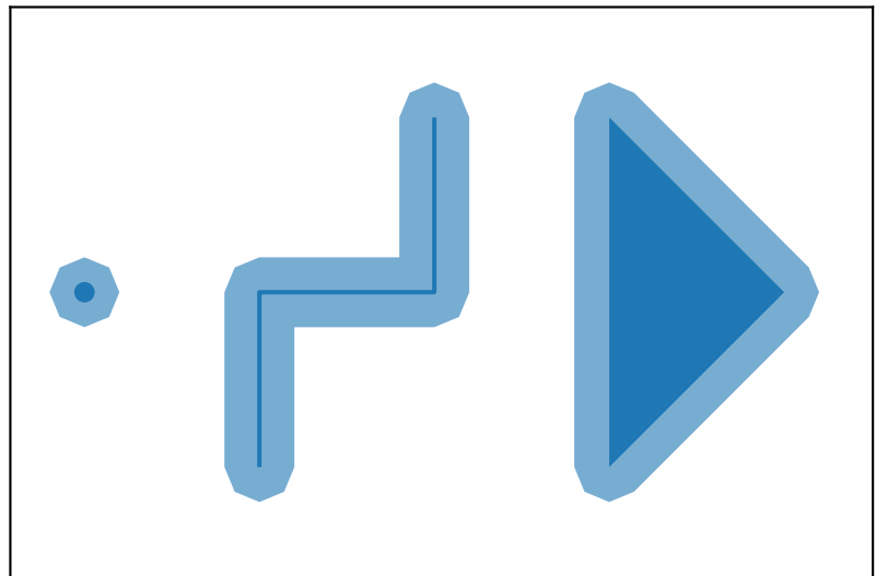
s.buffer(0.2, resolution=2)
