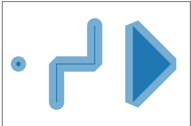
s.buffer(0.2, join_style=3)
