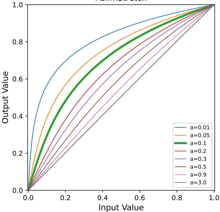
AsinhStretch
