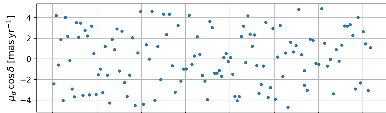
ICRS
