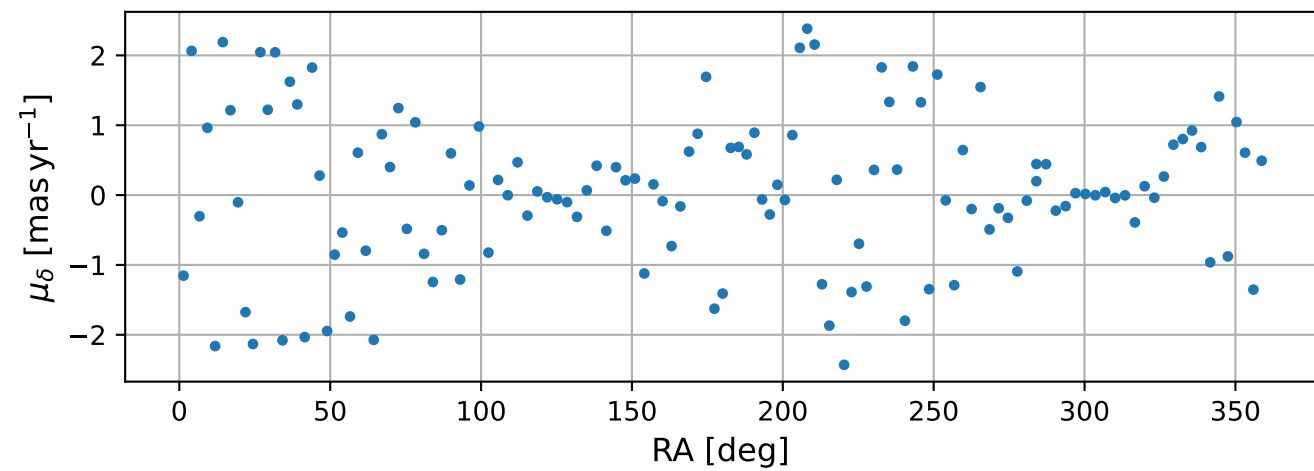
ICRS
