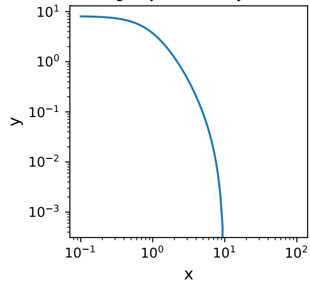
KingProjectedAnalytic1D
